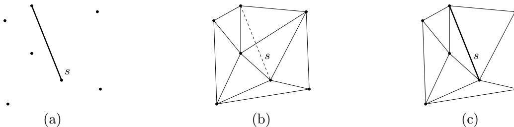
Figure 1: (a) The point set P of 7 points and segment set S of 1 segment s . (b) \text{DT}(P) = \text{CDT}(P, \emptyset) . (c) \text{CDT}(P, S) .
