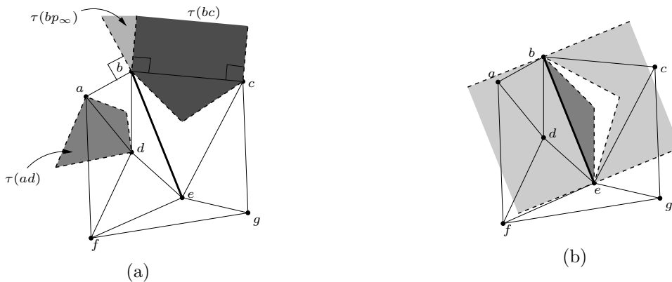
Figure 3: (a) The kernels of edges ad, bc , and bp_\infty . (b) The kernel of the edge be ; the darker part lies in the primary sheet, and the lighter part lies in the secondary sheet \Sigma_{be} .
