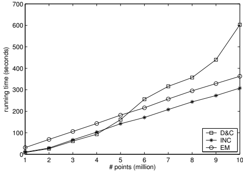
Figure 10: Delaunay triangulation results on the Kuzmin distribution.
